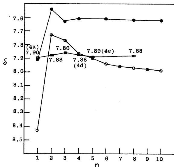
Fig. 3. Relationship between the chemical shifts (H-8 of 2 and 4 and H-6 of 6 ) and the carbon numbers ( n ) of polymethylene chains in D_2O at 27^\circ C using sodium 3-(trimethylsilyl)propionate-2,2,3,3- d_4 as the internal standard; the concentrations of compounds: <1 mg/0.5 ml ( D_2O ). The values of chemical shifts of 2 and 6 are summarized in Table 2.
