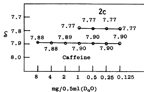
Fig. 6. Relationship between the chemical shifts (H-8 of 2c and caffeine) in D_2O at 27^\circ C using sodium 3-(trimethylsilyl)propionate-2,2,3,3- d_4 as the internal standard and the concentrations of 2c and caffeine.
